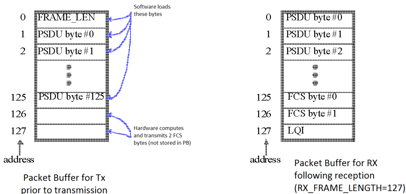
Figure 8-12. Packet buffer architecture
