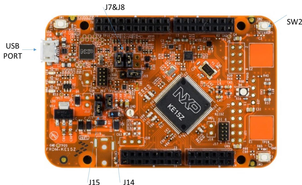
Figure 2. FRDM-KE15Z Board
