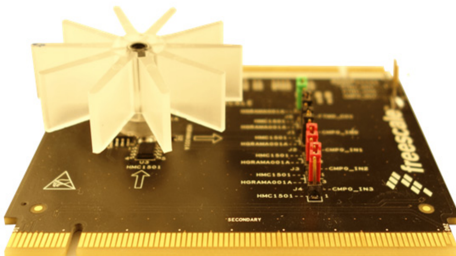
Figure 9. The TWR-FLOW-MAG board with a paddle wheel as the encoder
