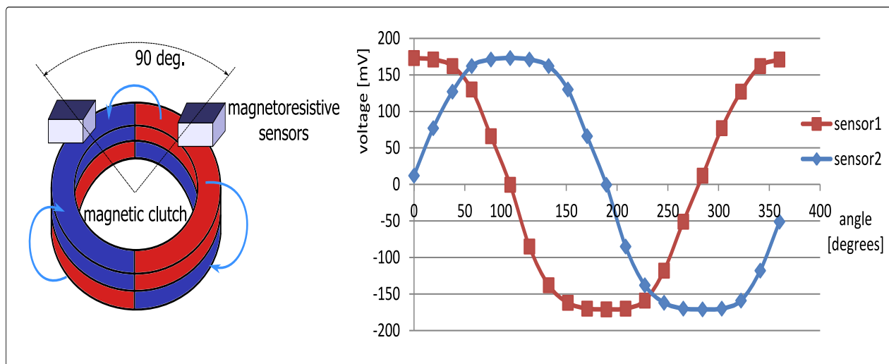
Figure 2. The magnetic sensor-based encoder principle at work
