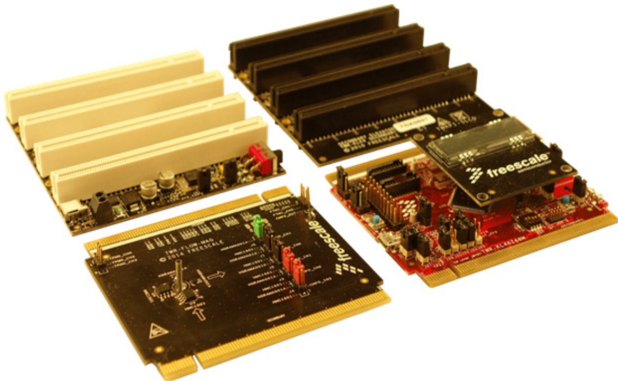
Figure 8. The accessory board TWR_FLOW_MAG
