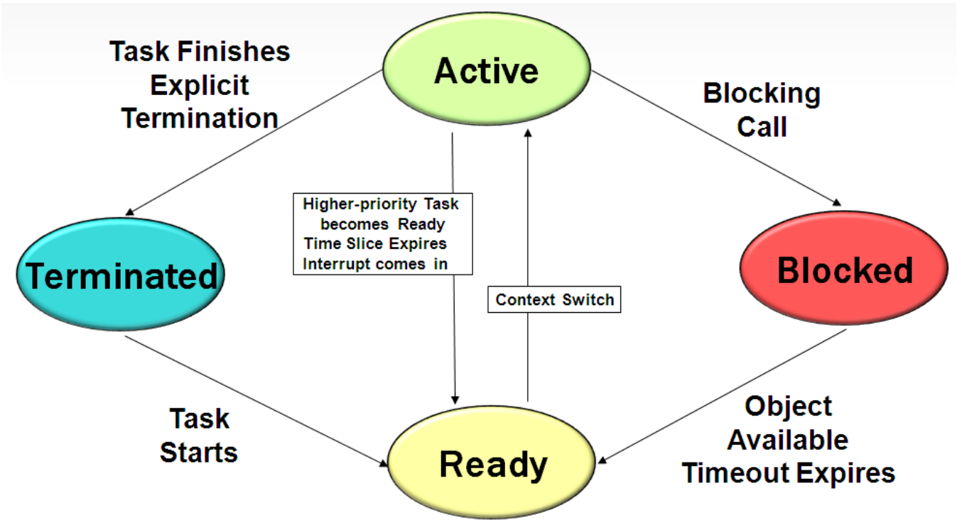
Figure 9. Task states
