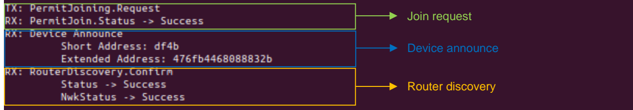
Figure 39. Board A, join request.
