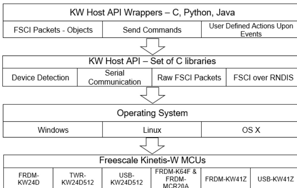
Figure 1. Kinetis Wireless Host Software System Block diagram.
